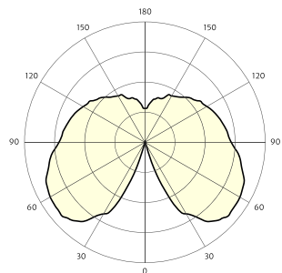
Smoked bulb - Light Intensity distribution
