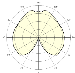
Clear bulb - Light Intensity distribution
